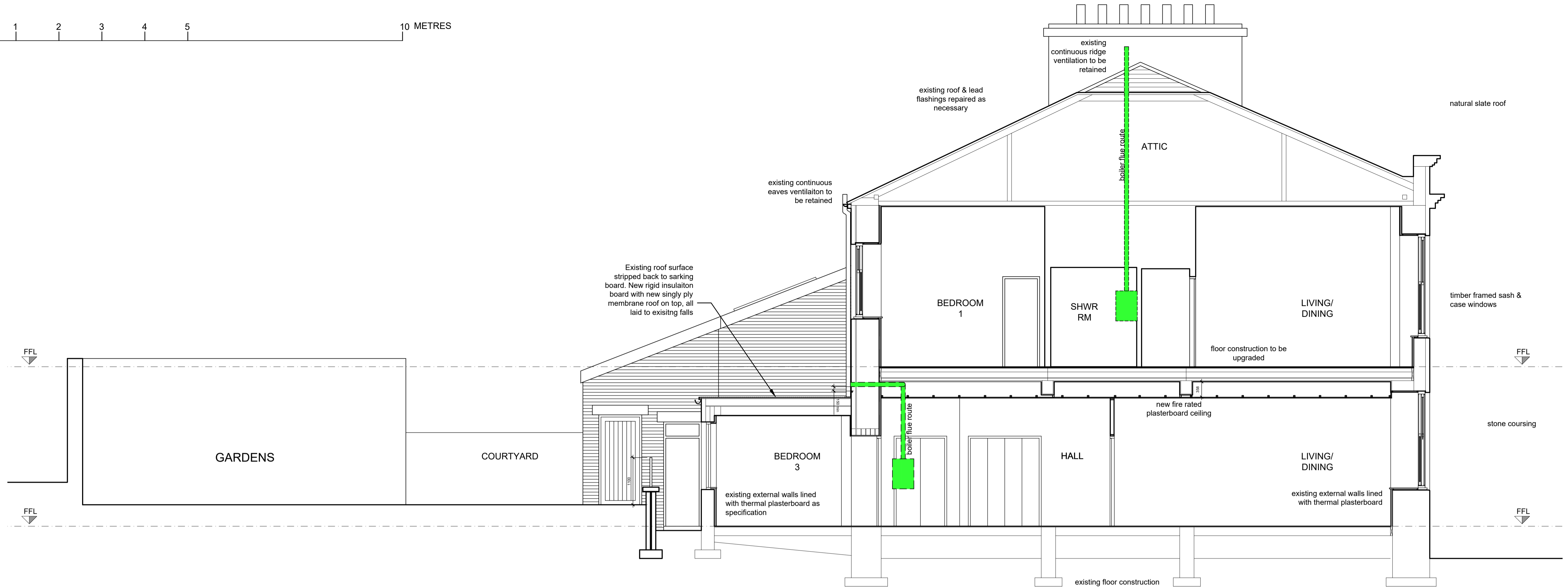
SECTION A - A AS PROPOSED
