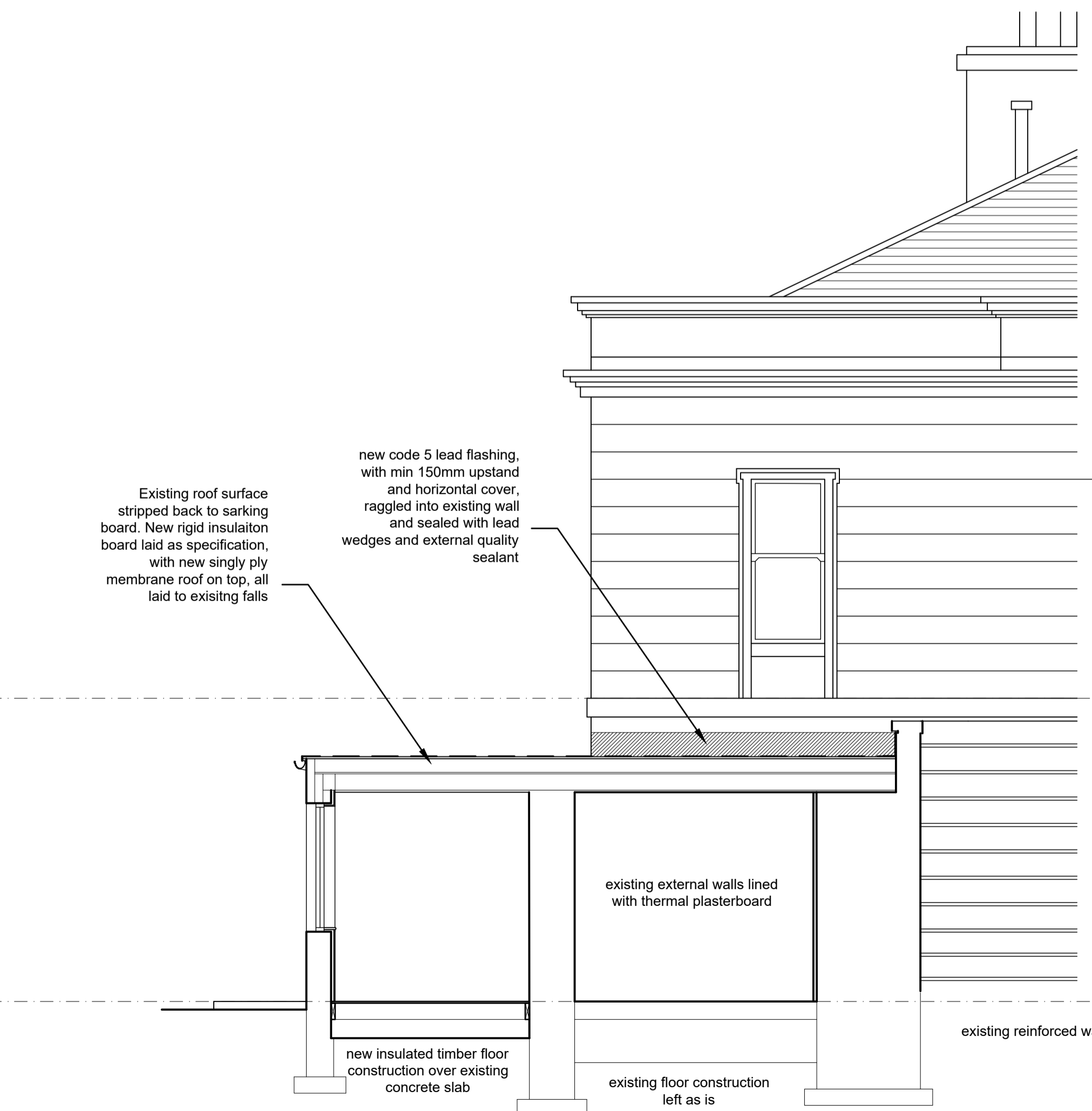
SECTION C - C AS PROPOSED
