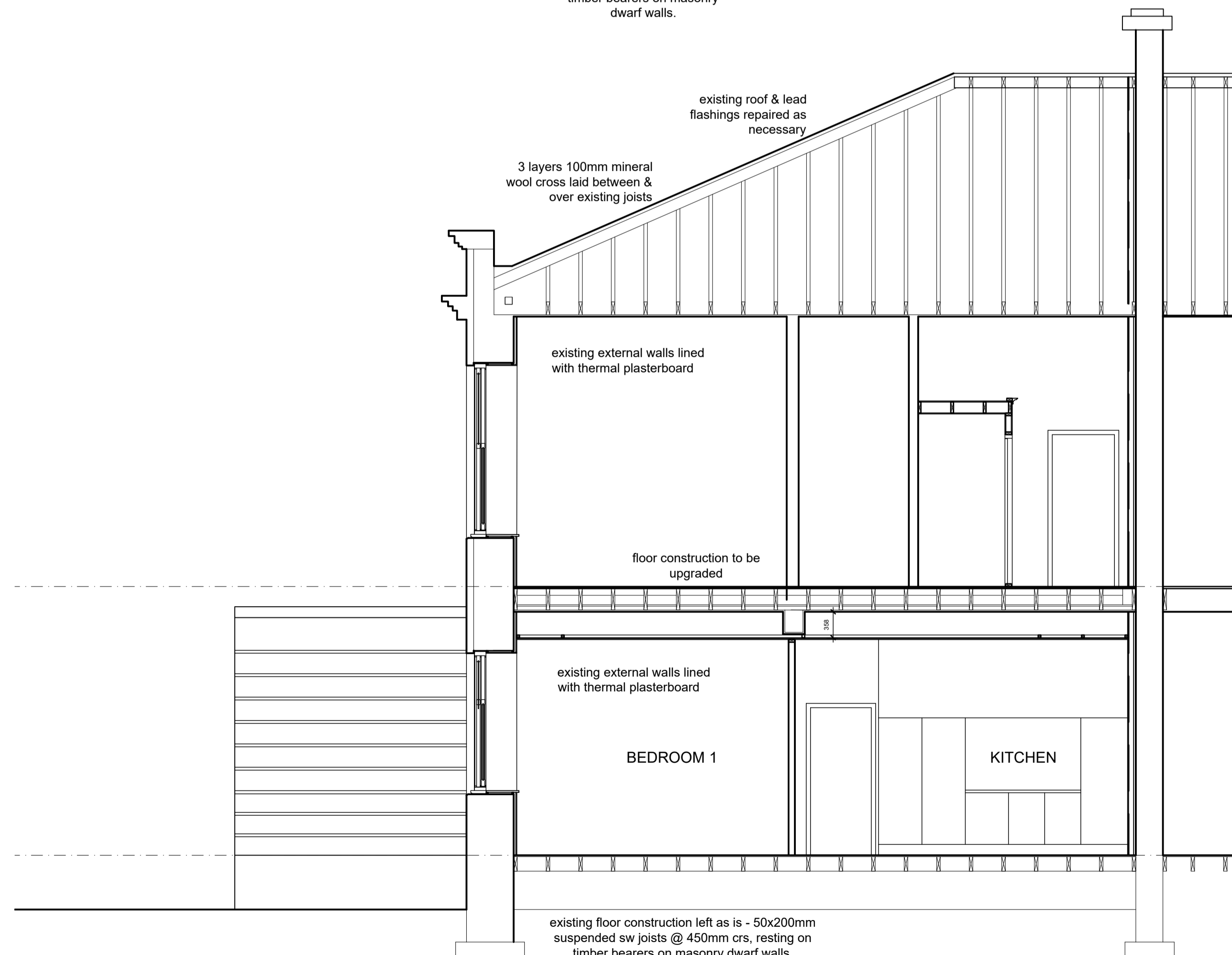
SECTION B - B AS PROPOSED
