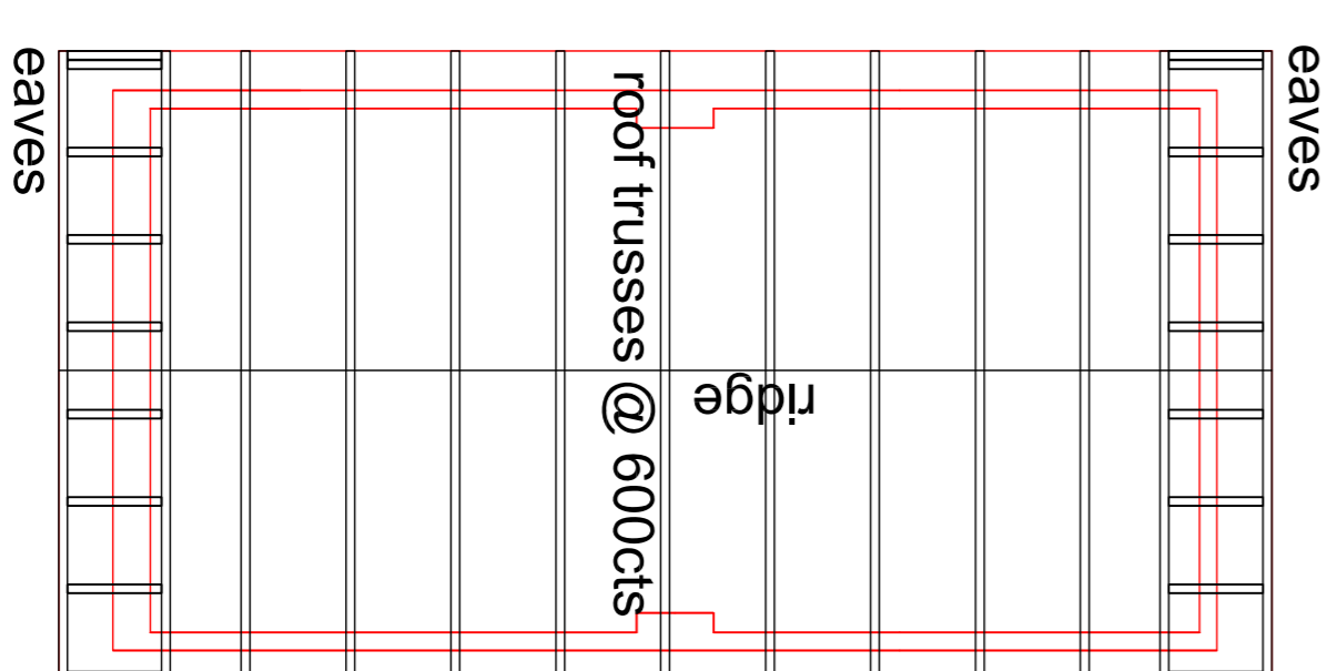
Roof Plan
