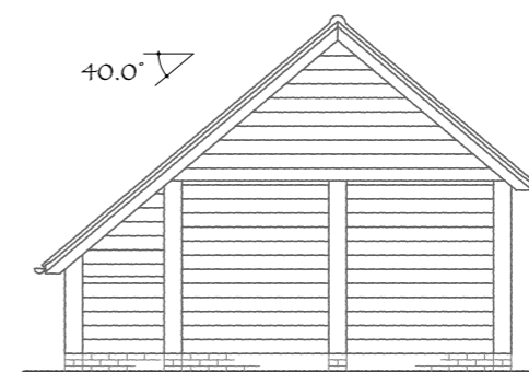
SOUTH ELEVATION
