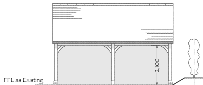
EAST ELEVATION
