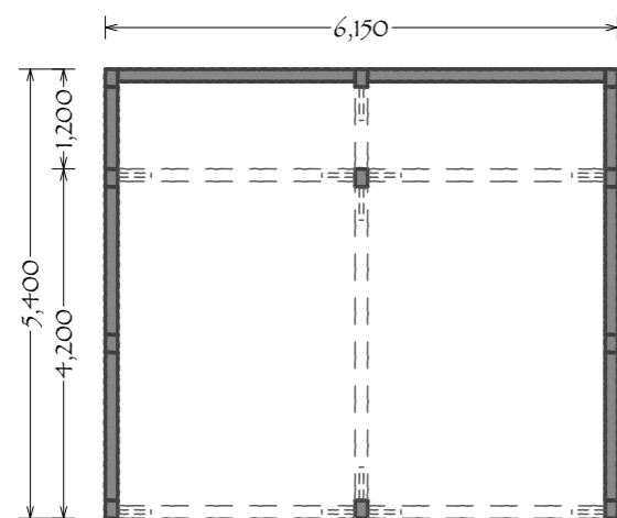
FLOOR PLAN
