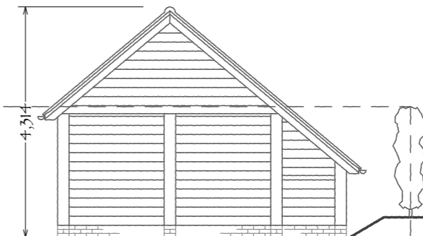
NORTH ELEVATION
