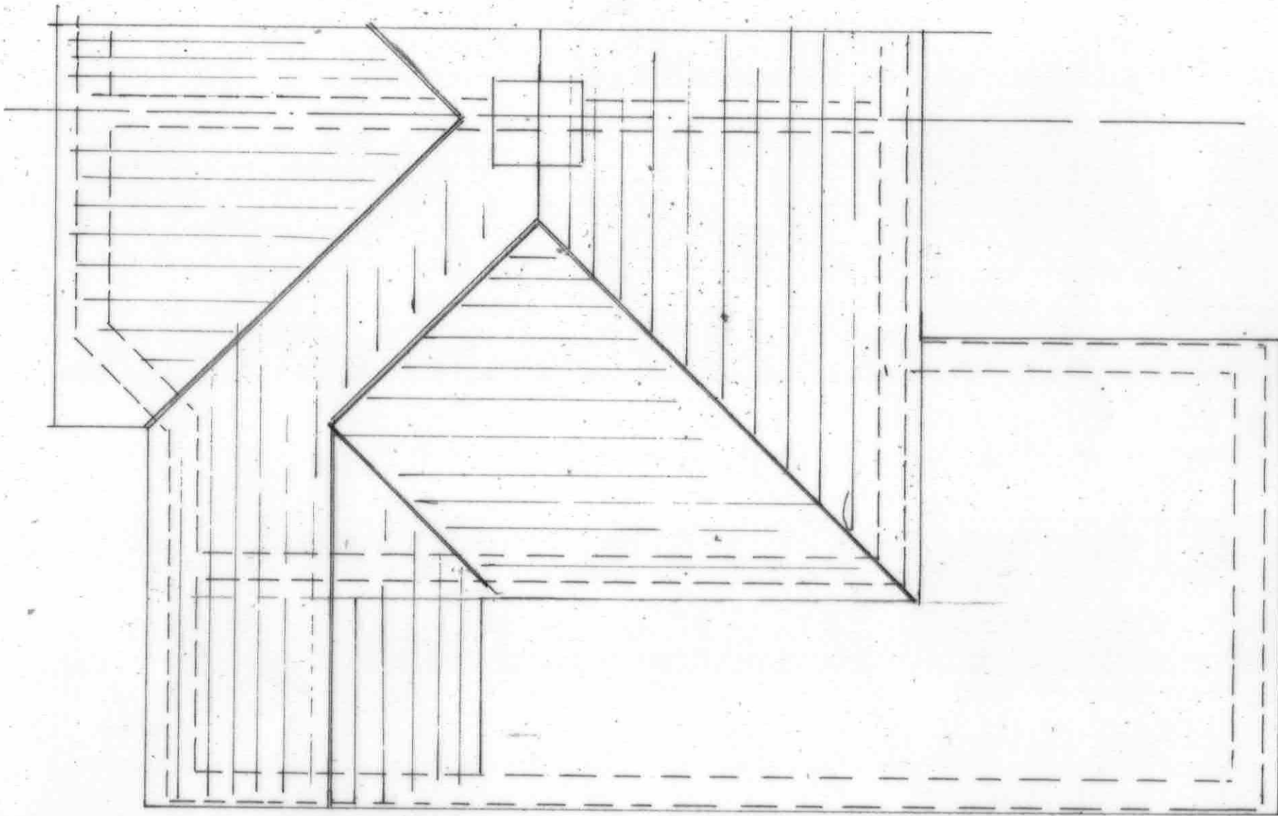
Roof Plan
