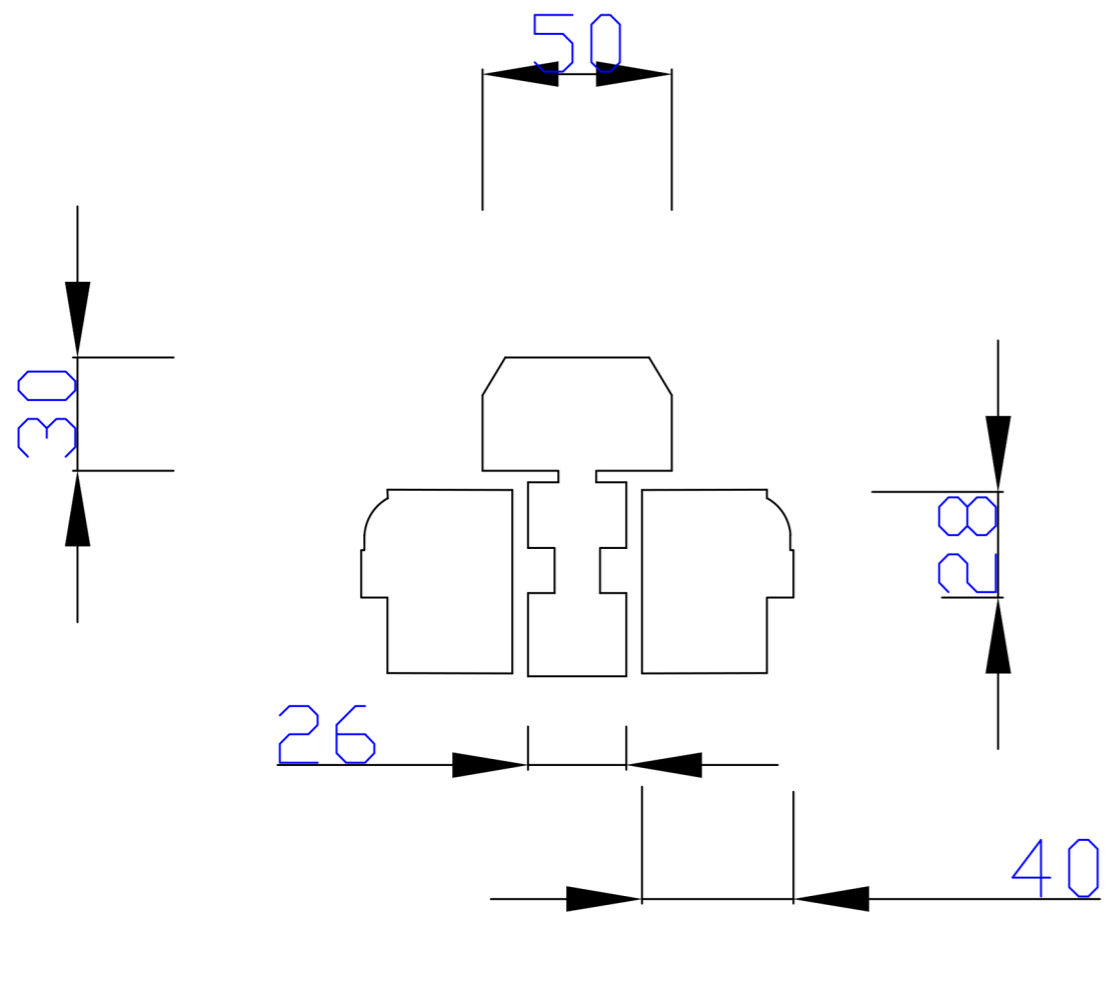
Window section MP04 scale 1;2 @ A3
