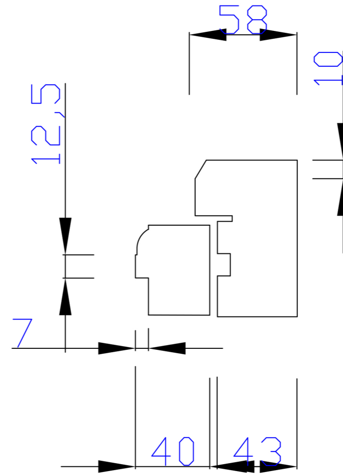
Window section MP04 scale 1;2 @ A3
