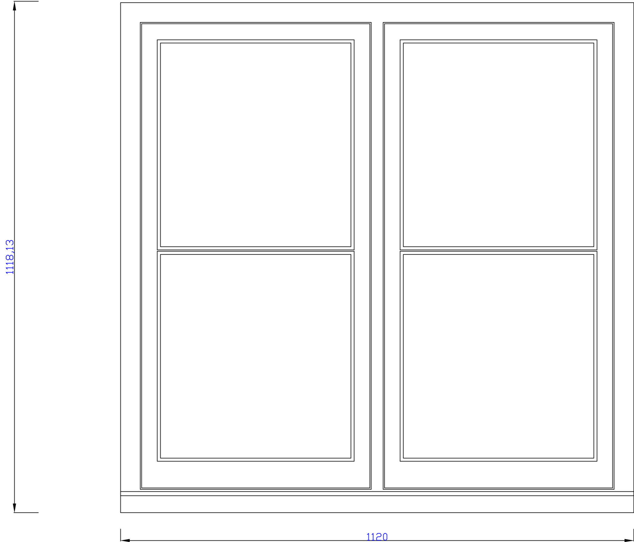
Window elevation MP02 1;5 @ A3
