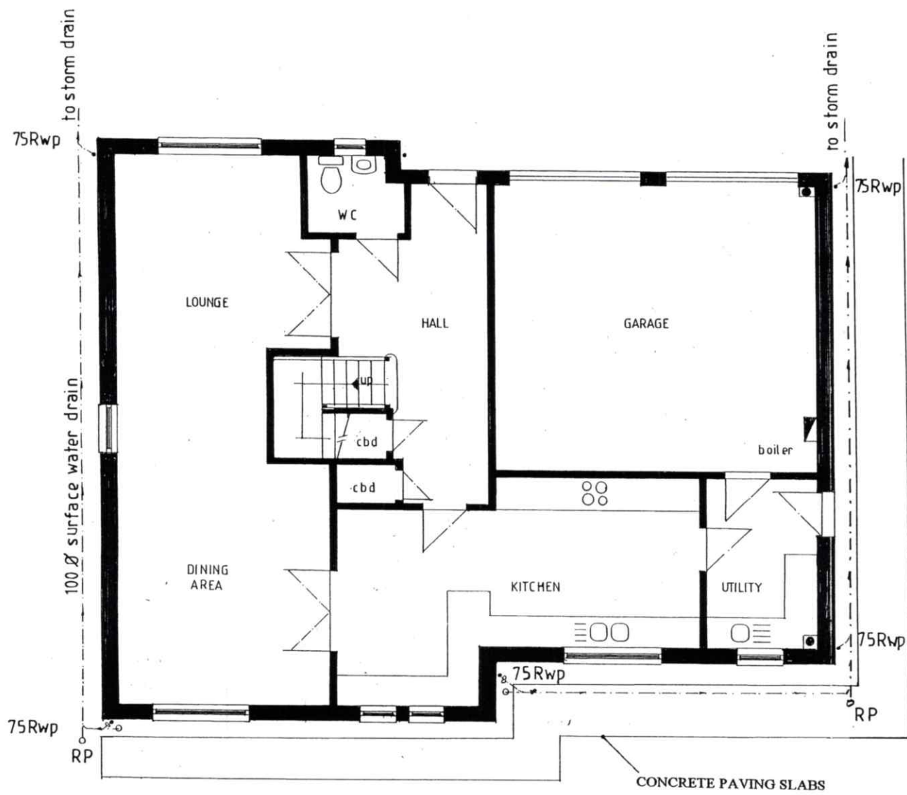
GROUND FLOOR PLAN as existing
