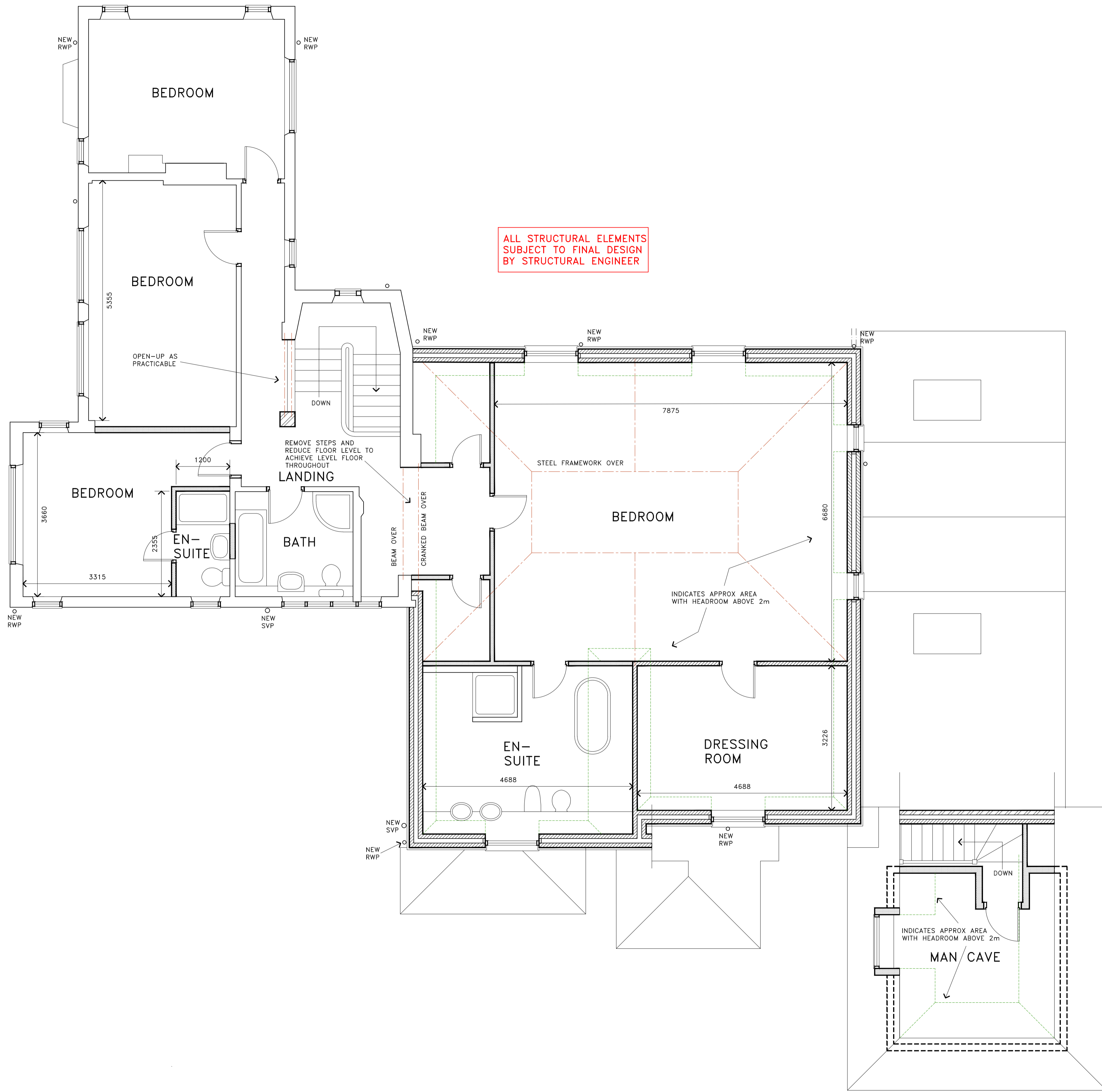
PROPOSED FIRST FLOOR PLAN 1:50
