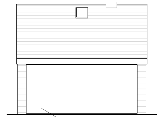
South Elevation
