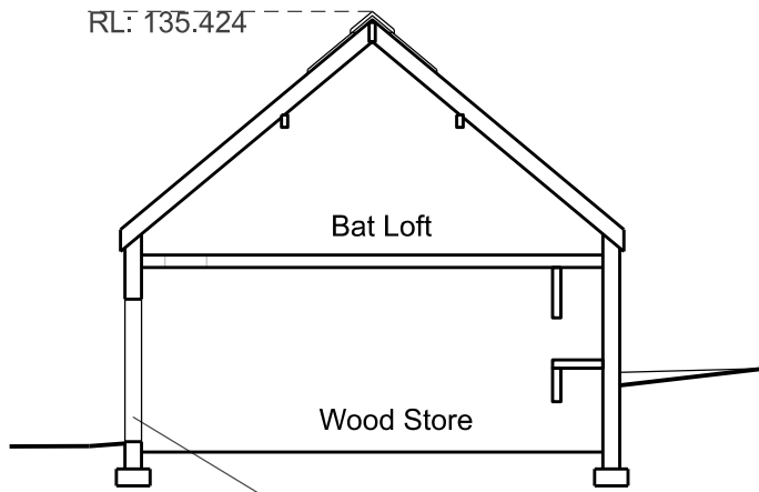
Proposed Section
