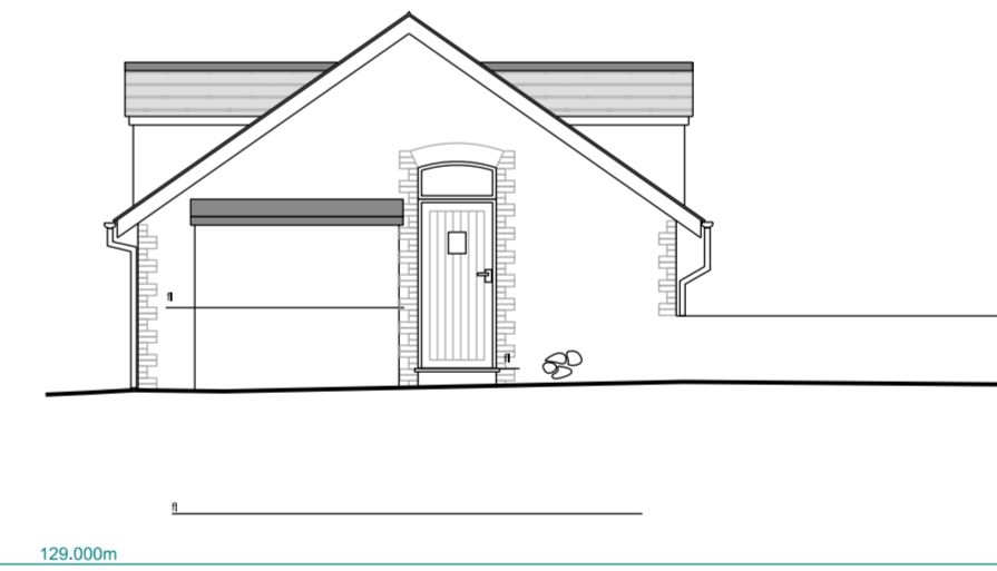
North Elevations
