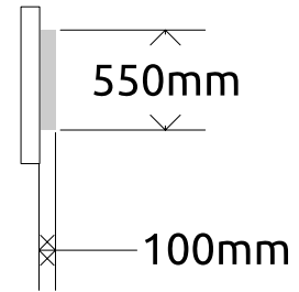
Side elevation of light box
