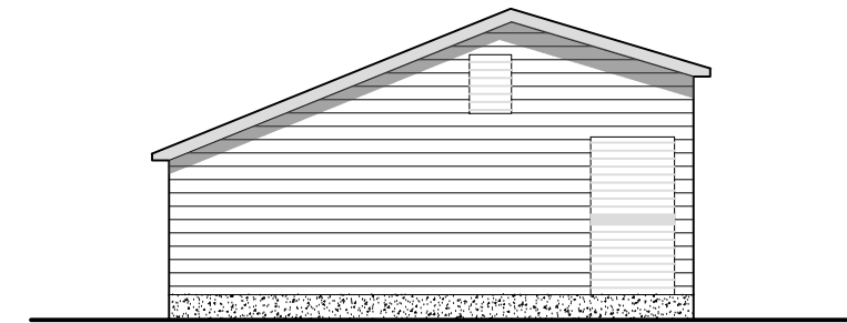
WEST ELEVATION 1:100
