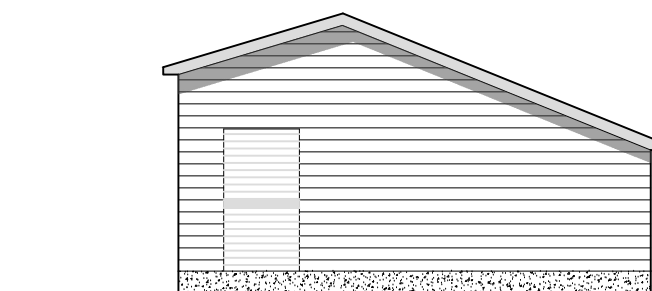
EAST ELEVATION 1:100
