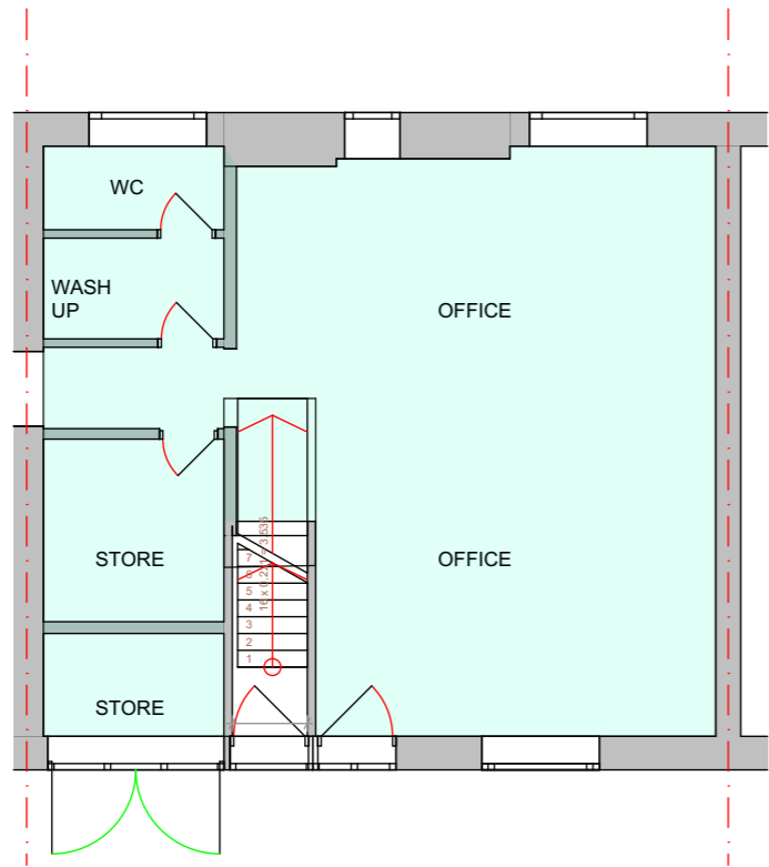
GROUND FLOOR 1:100
