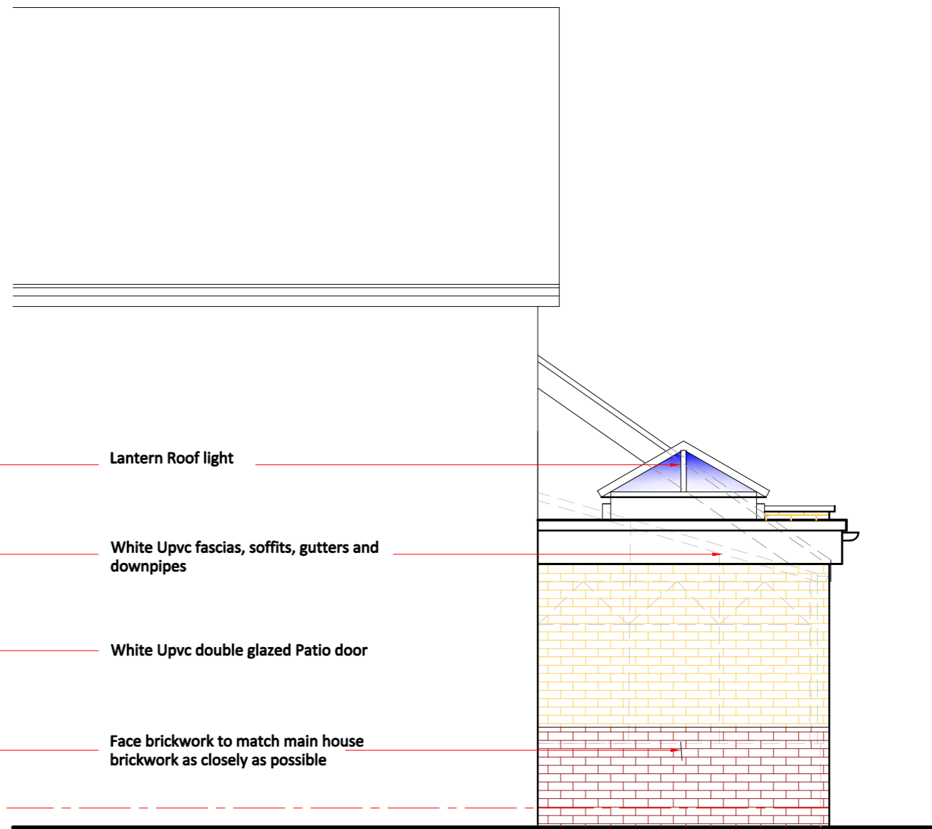
North Elevation
