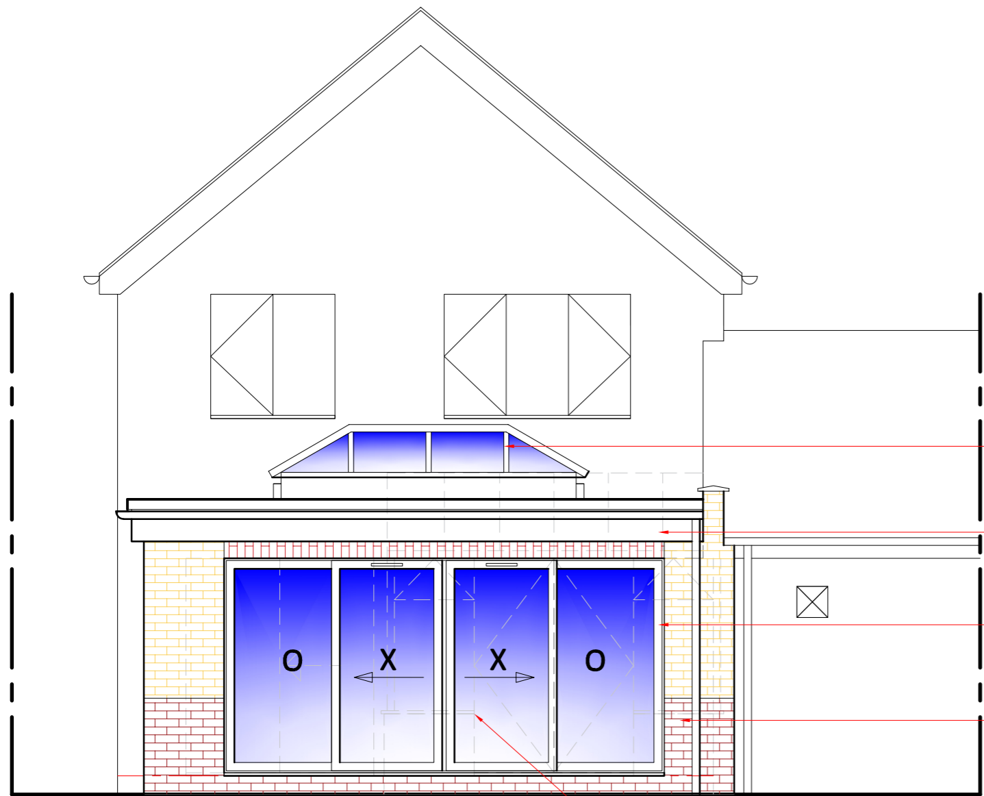
West Elevation
