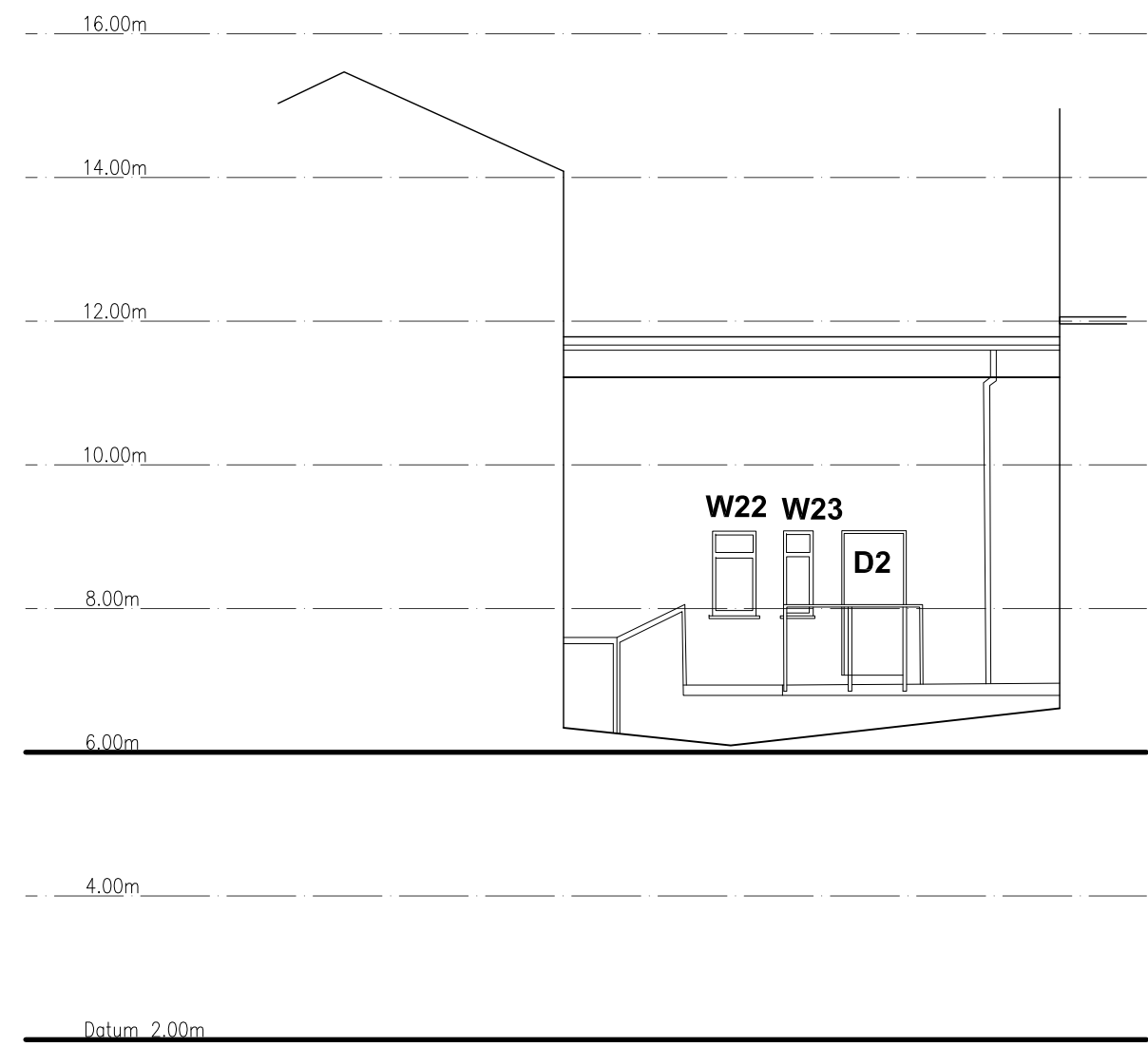
02 EXISTING ELEVATION D-D
