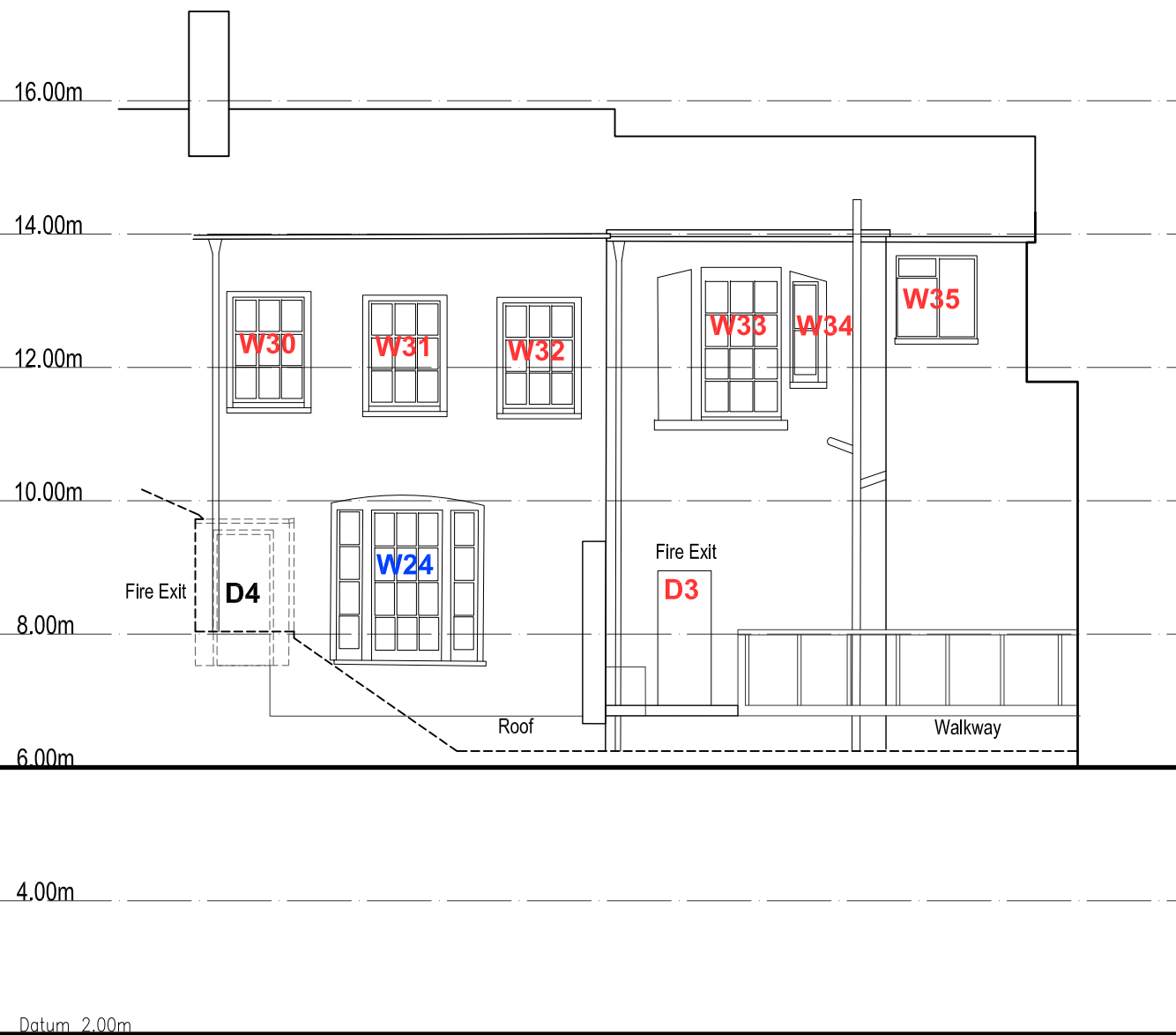
01 EXISTING ELEVATION C-C
