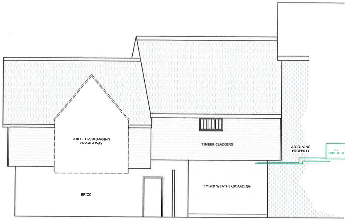
REAR ELEVATION (WEST)
