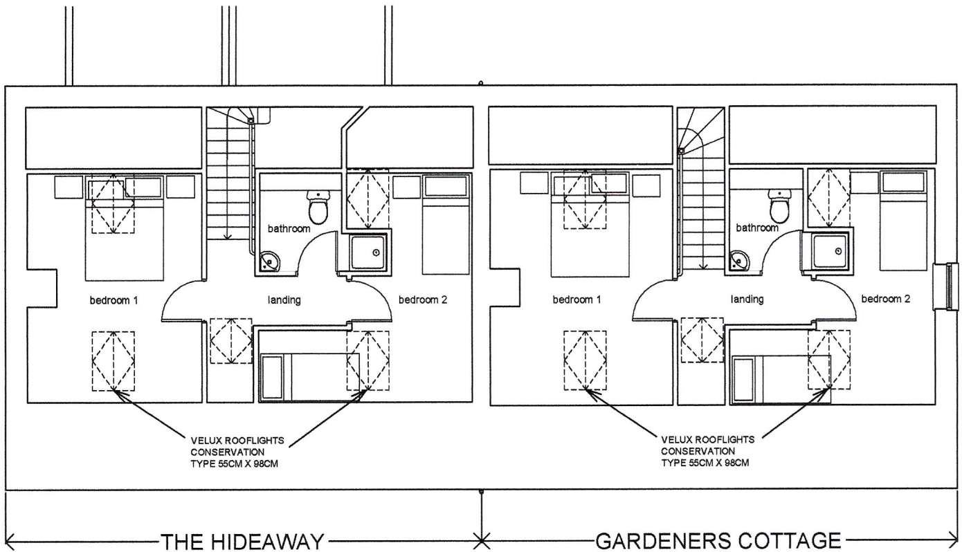
PROPOSED FIRST FLOOR PLANS
