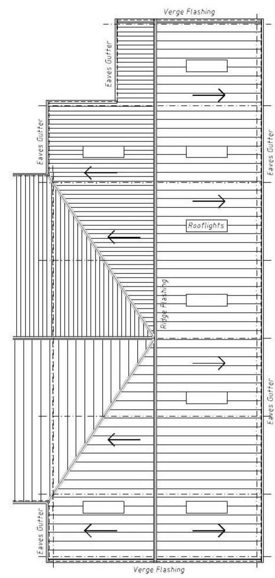
Roof Plan 1:200
