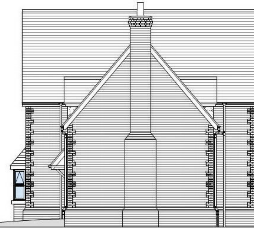
West elevation - as existing
