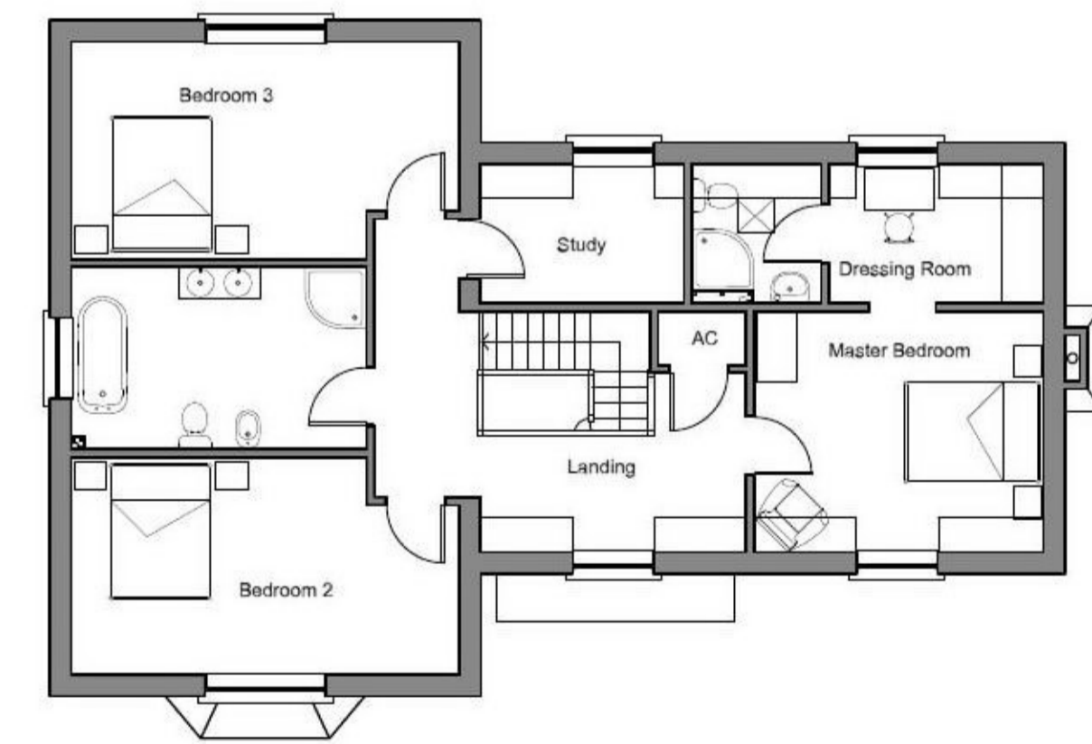
First floor plan - as existing
