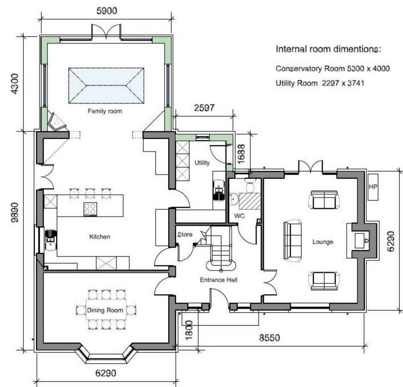
Ground floor plan - as proposed
