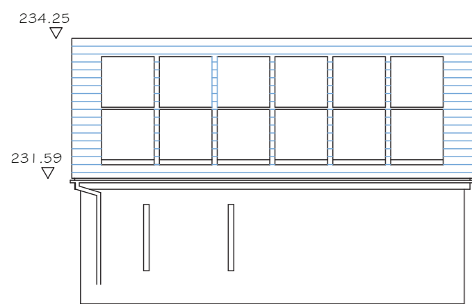
WESTERN ELEVATION
