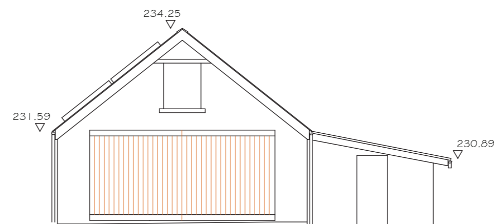
SOUTHERN ELEVATION
