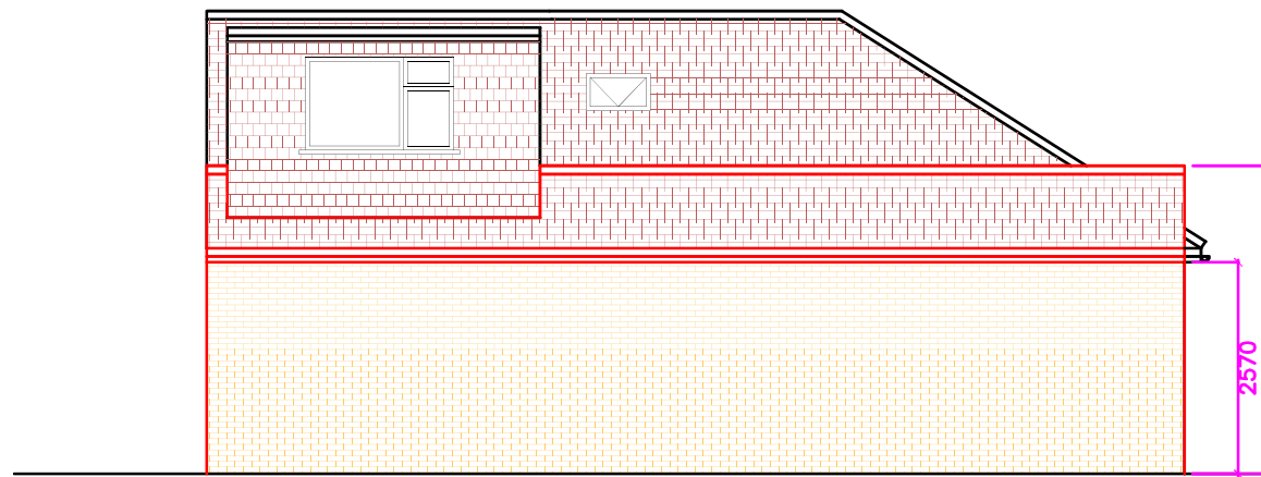
Proposed Side Elevation - A
