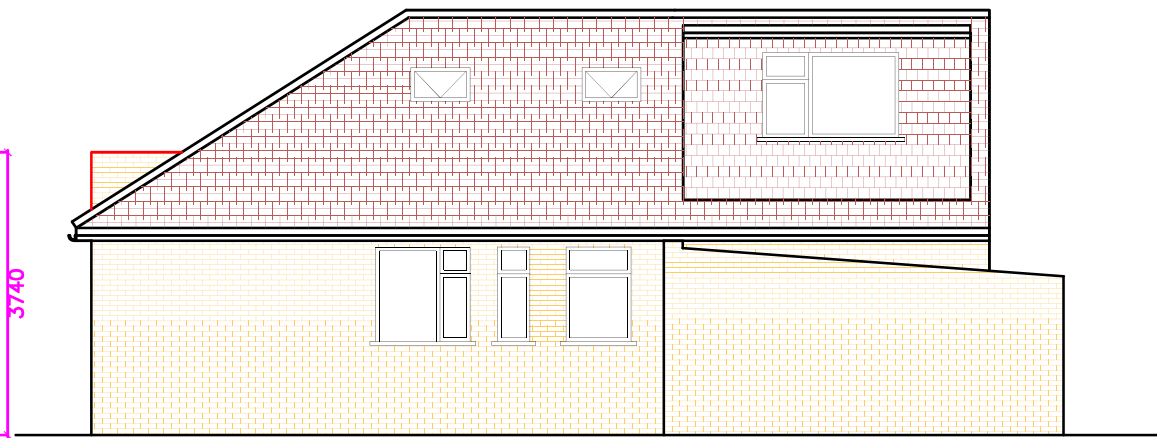
Proposed Side Elevation - B
