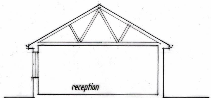
Section
