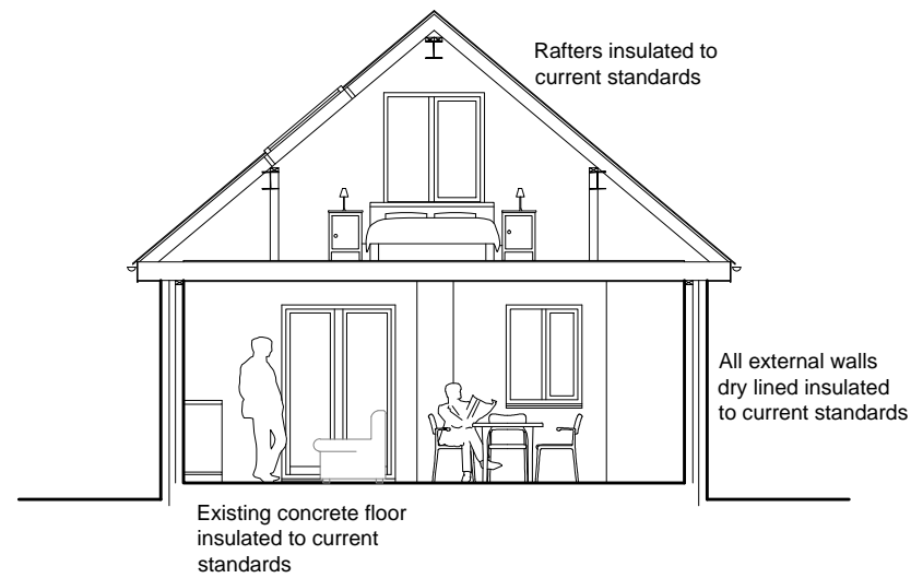
Proposed Section Scale 1:100
