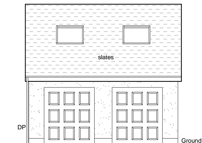
Existing East Elevation Scale 1:100
