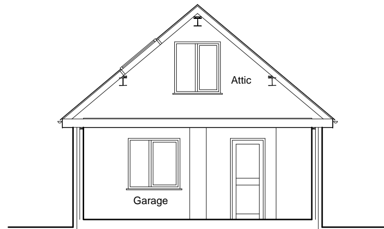
Existing Section Scale 1:100
