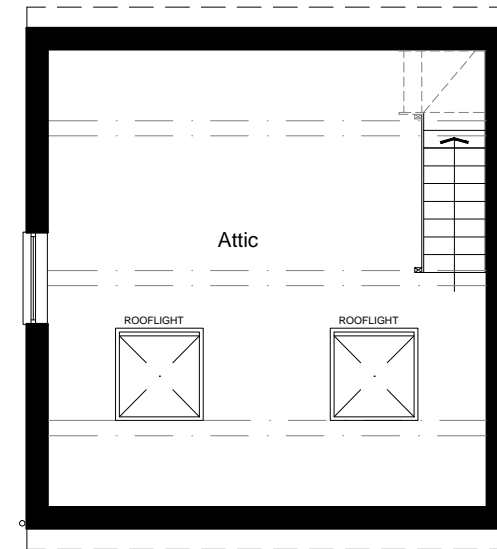
Existing Upper Floor Plan Scale 1:100
