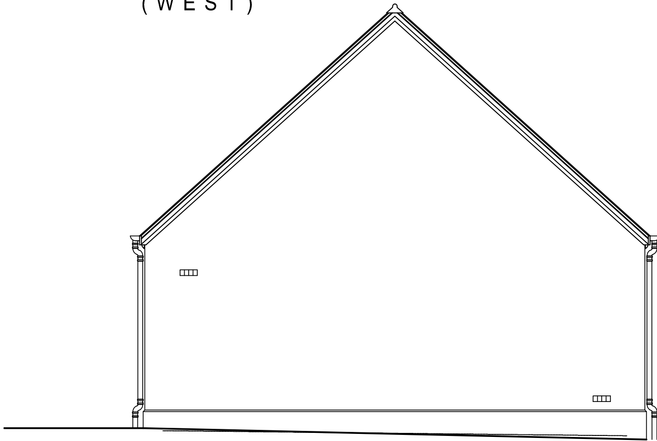
SIDE ELEVATION (NORTH)
