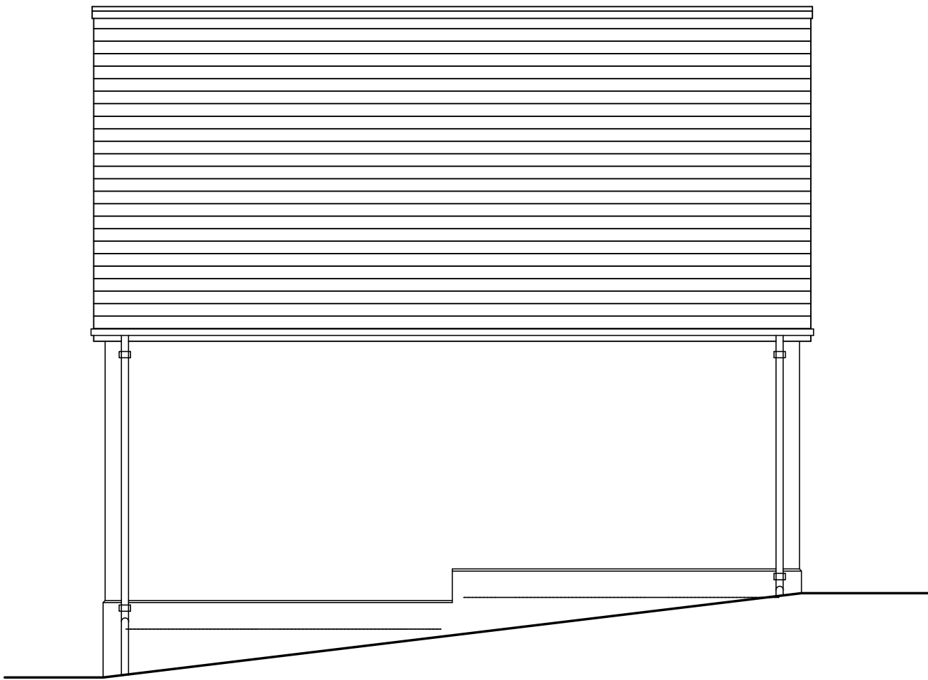
REAR ELEVATION (EAST)
