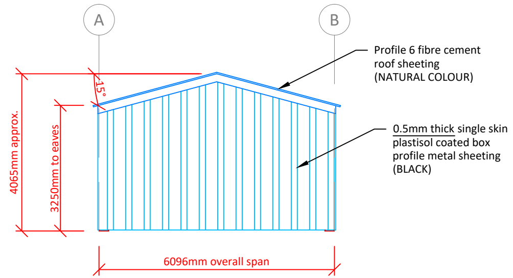
ELEVATION ACROSS GRIDLINE 1
