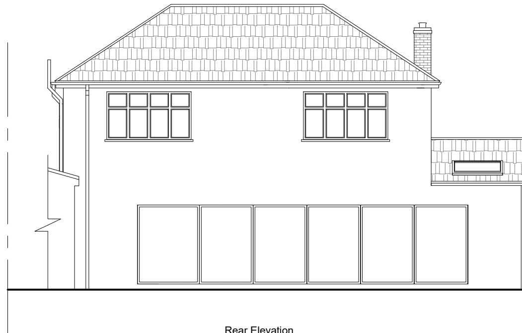
Rear Elevation
