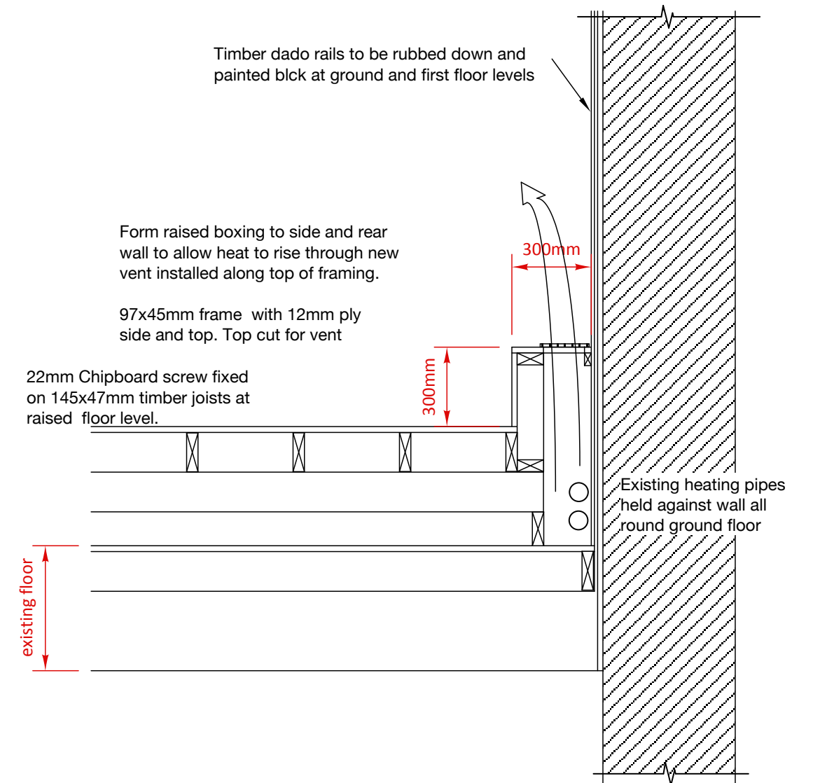
SECTION AT WALL VENT...
