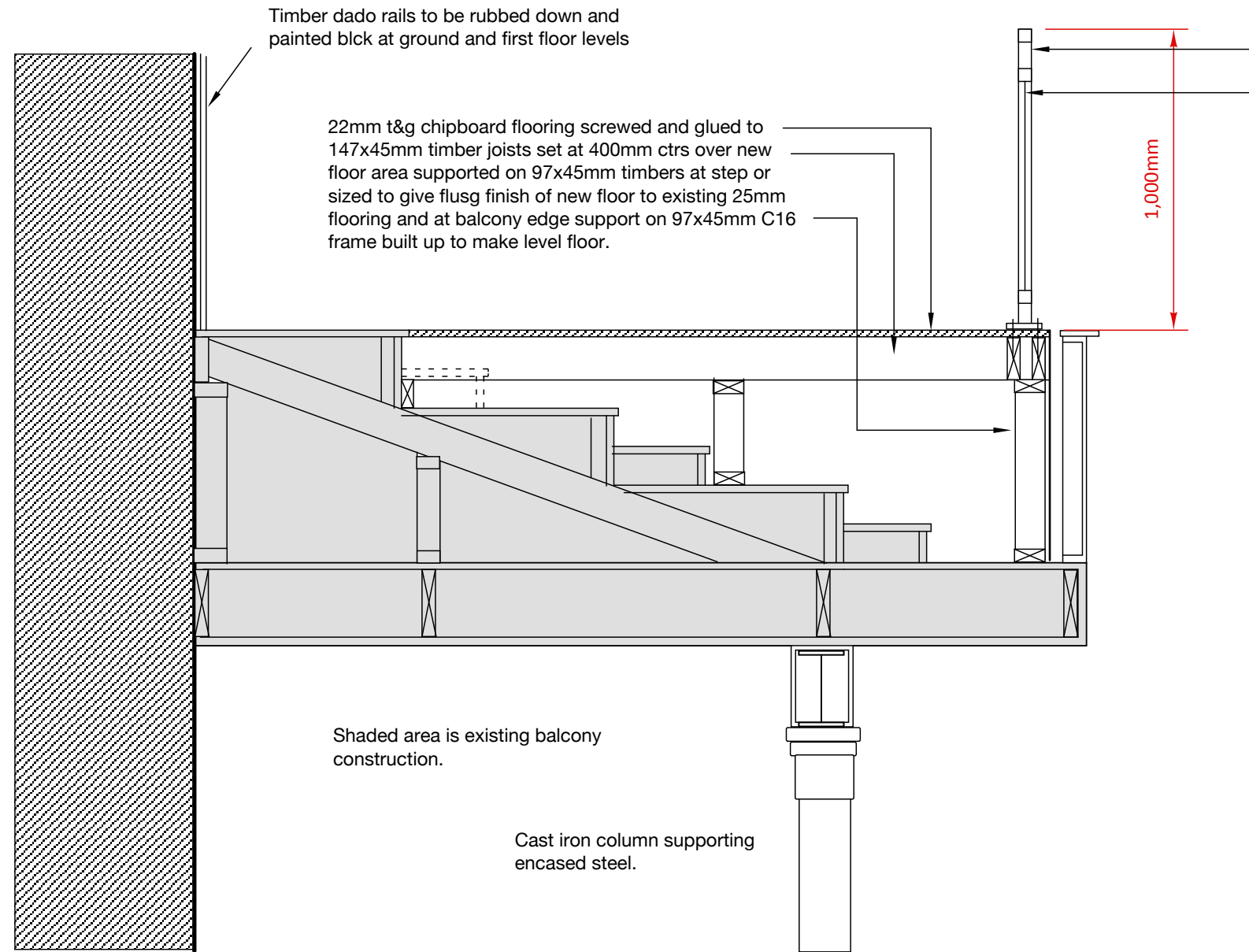
SECTION THROUGH BALCONY FOR NEW FLOOR...
