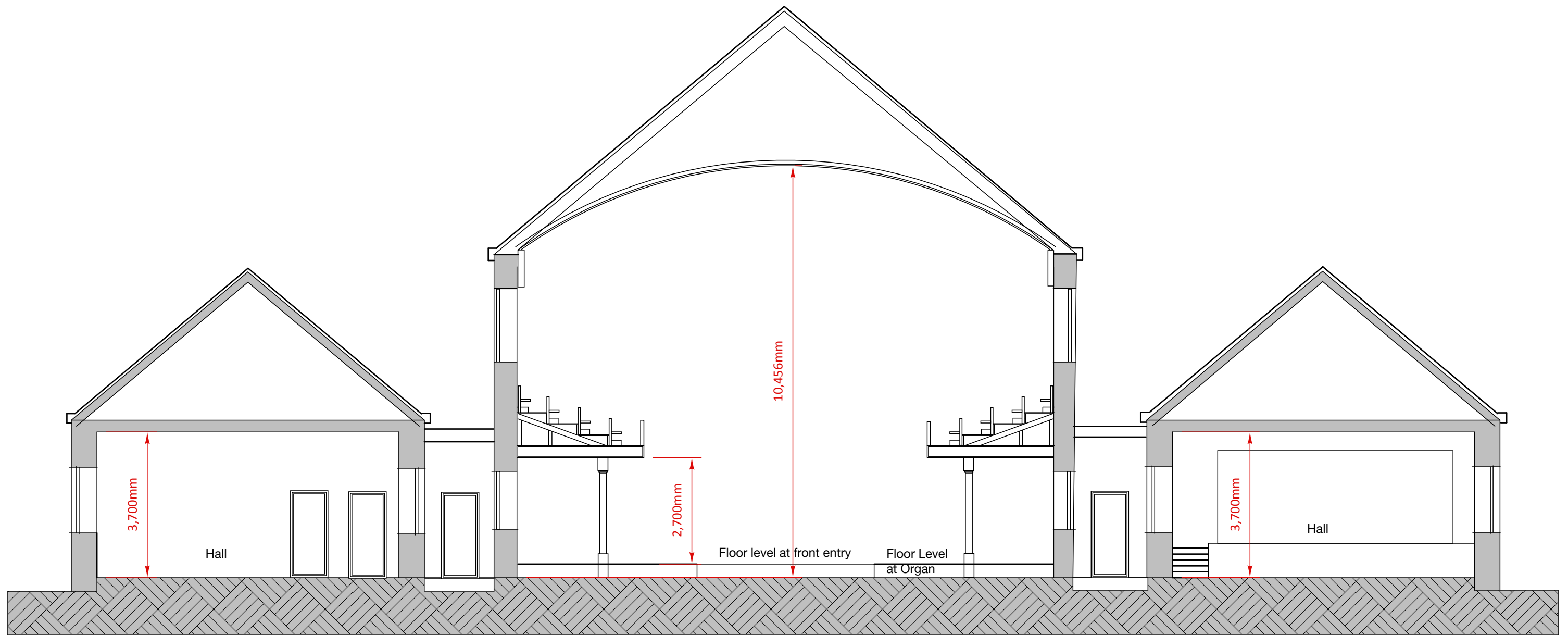
SECTION THROUGH CHURCH AND HALLS...
