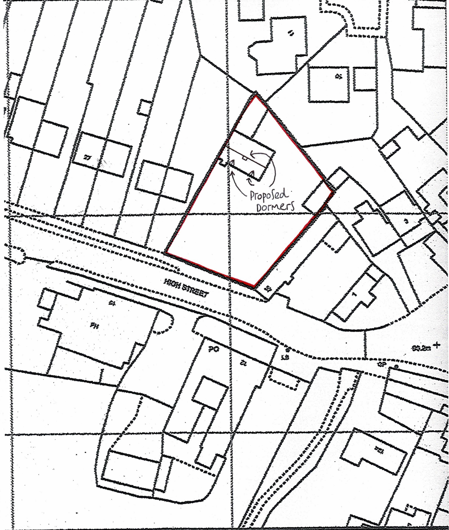
Block Plan 1:500 A4
