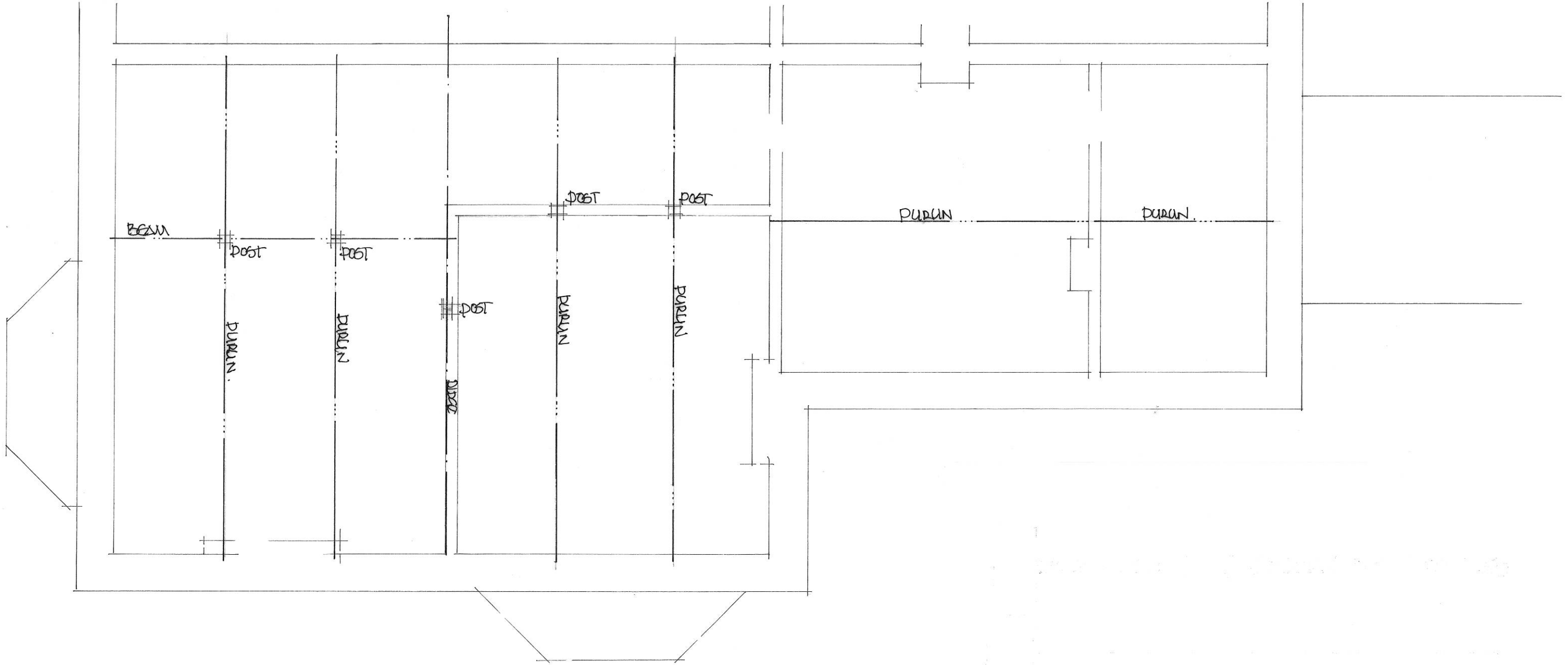
EXISTING ROOF PLAN. [MAIN ROOF] 1:50 @ A3.
