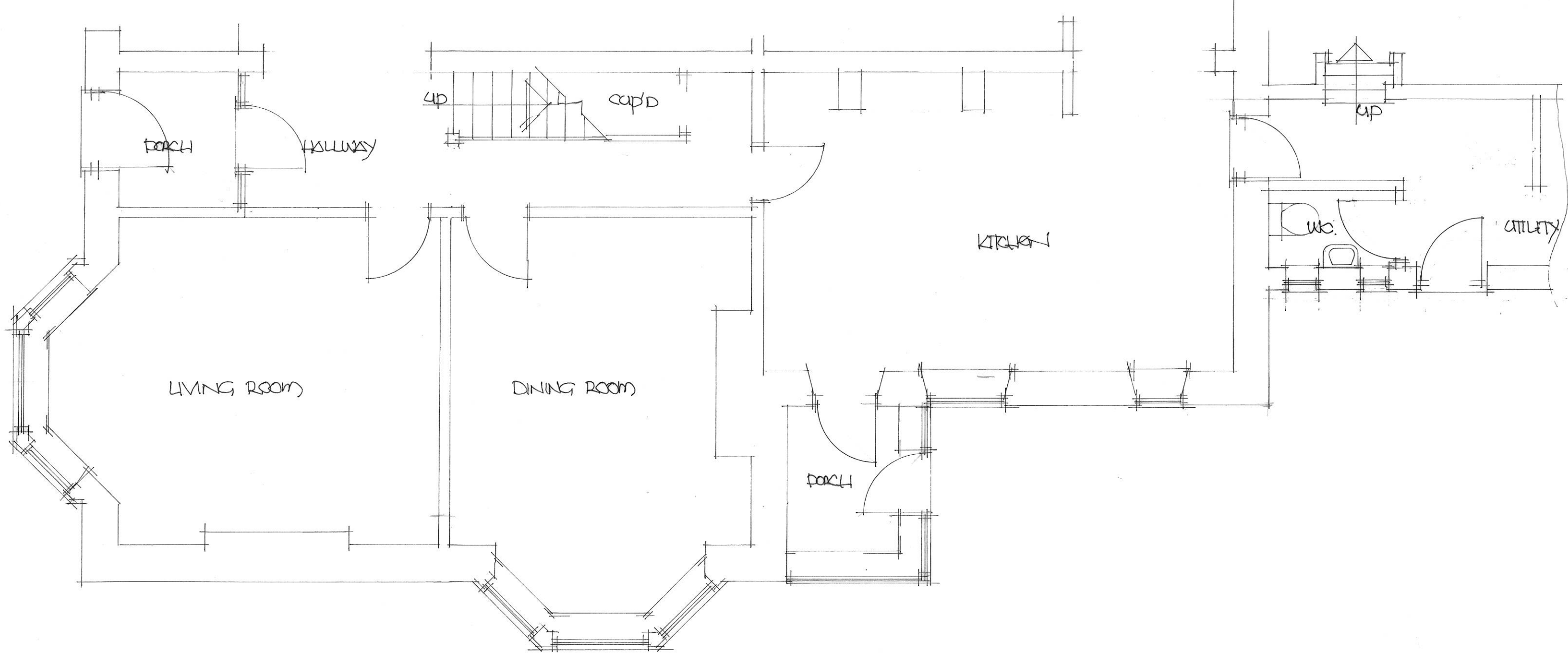
EXISTING GROUND FLOOR PLAN 1:50 @ A3 [NO 4 ASHPRED TERRACE.]
