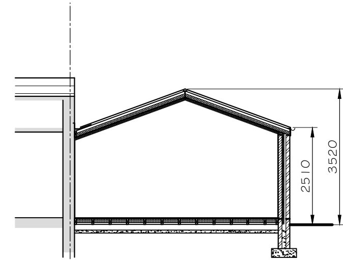
PROPOSED SECTION (1:100)
