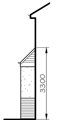
EXISTING SIDE ELEVATION TO No 15 (1:100)
