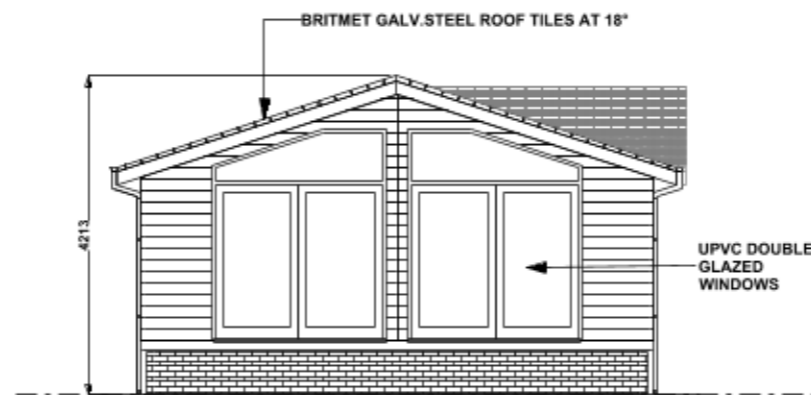
04 PROPOSED WEST ELEVATION
