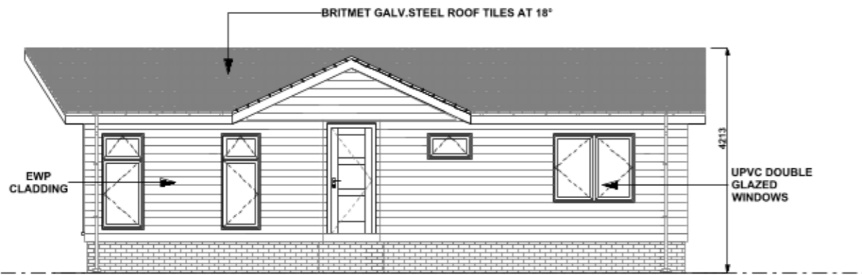
02 PROPOSED SOUTH ELEVATION
