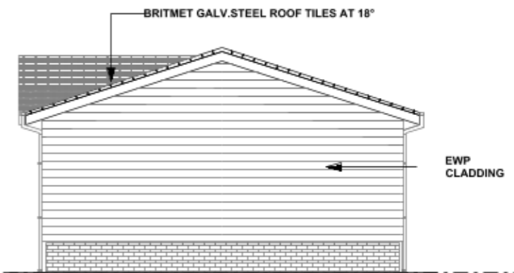
05 PROPOSED EAST ELEVATION
