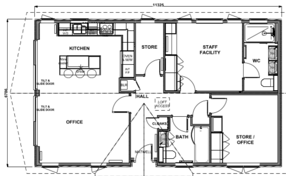
01 PROPOSED GROUND FLOOR PLAN
