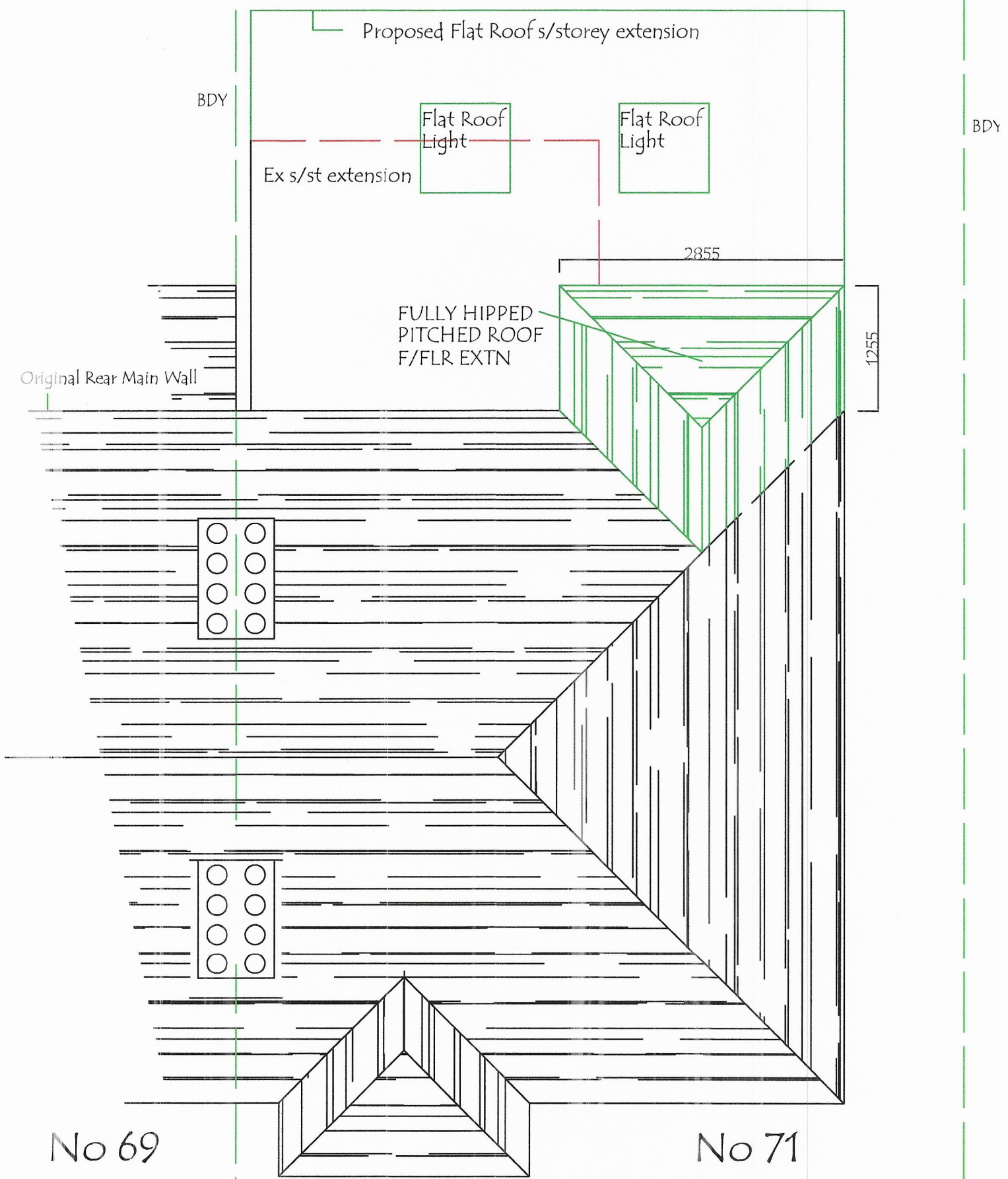
ROOF FLAN - AS PROPOSED
