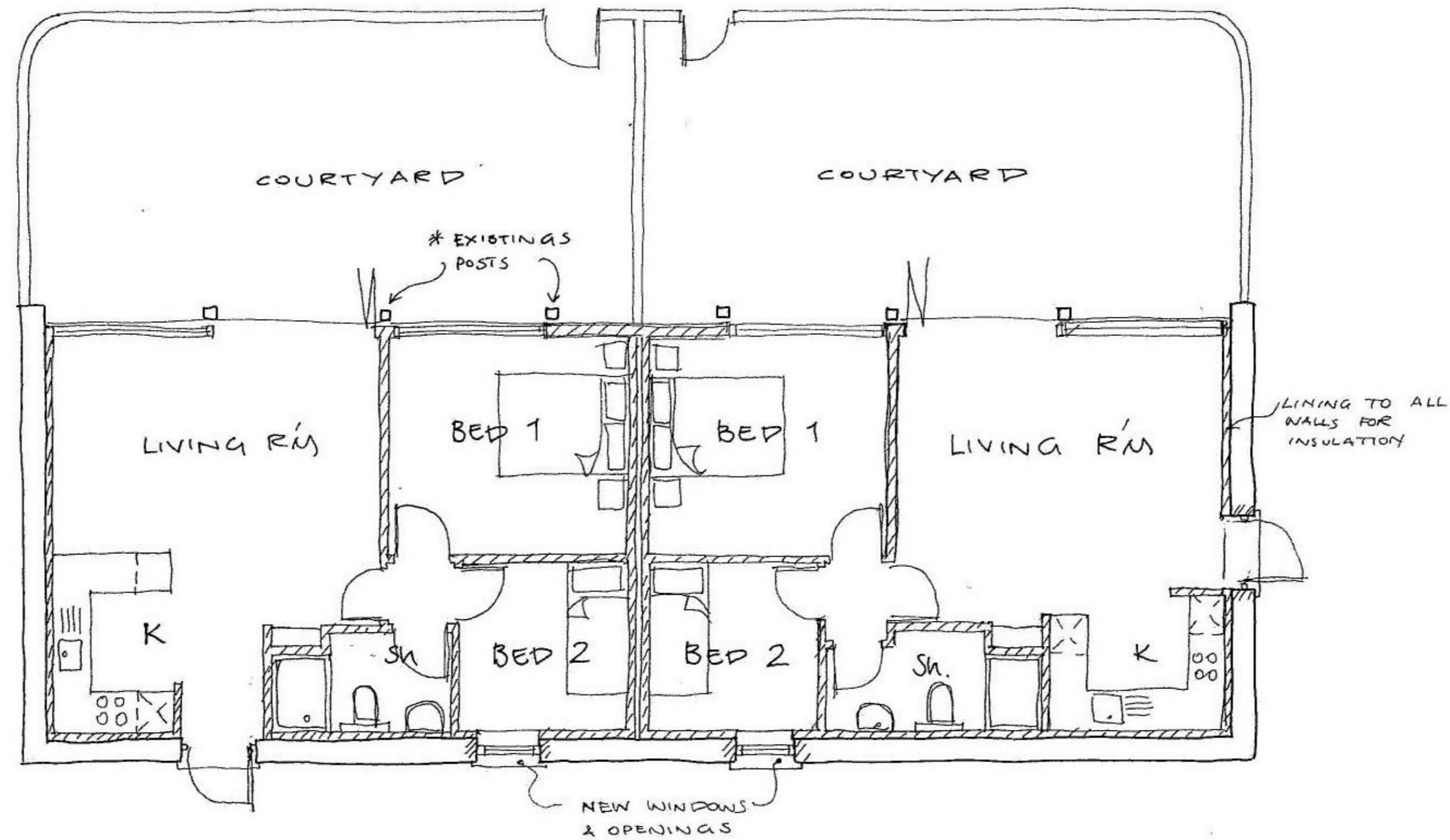
FLOOR PLAN ~ 1:100 as proposed ~
