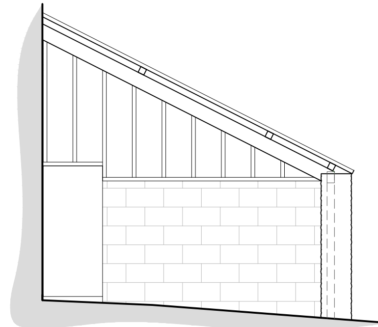
PROPOSED SECTION
