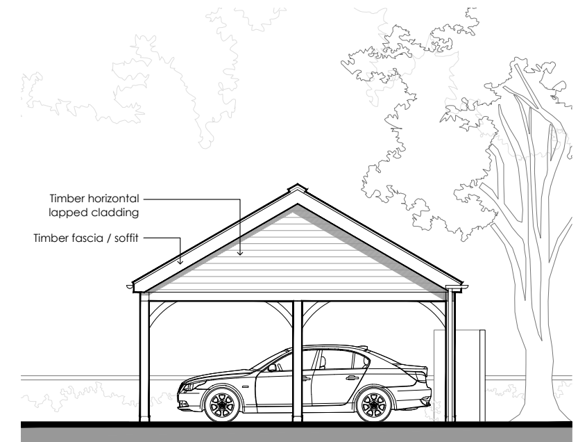
WEST ELEVATION
