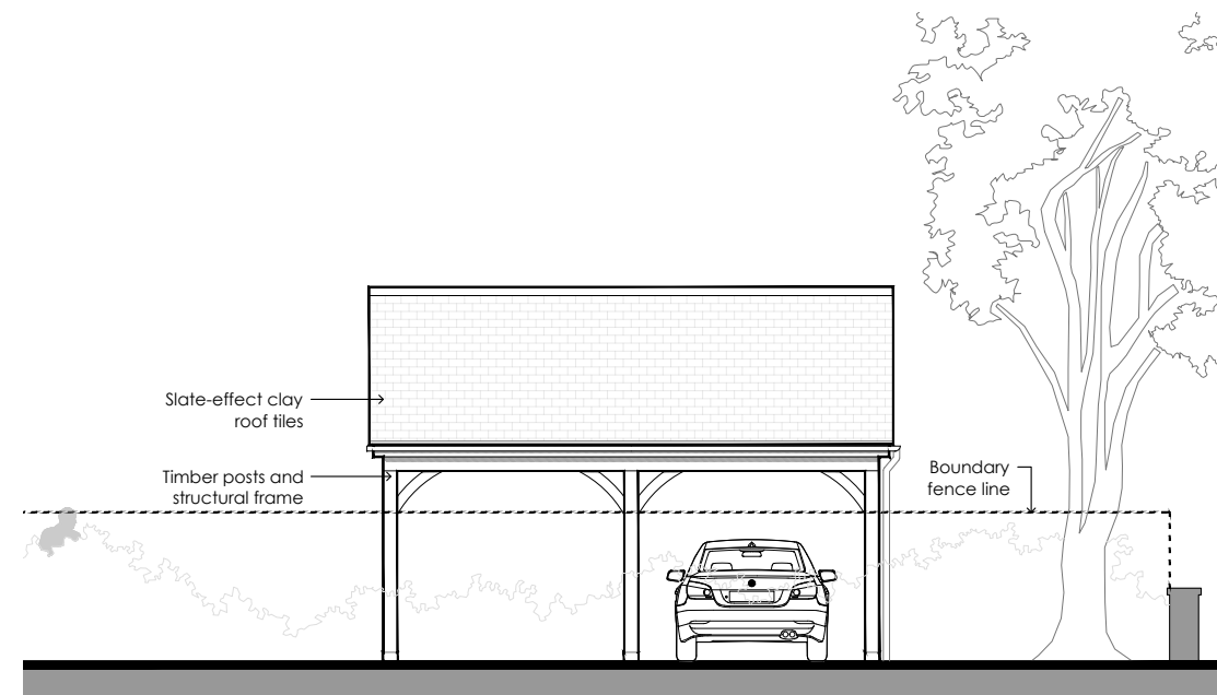
SOUTH ELEVATION
