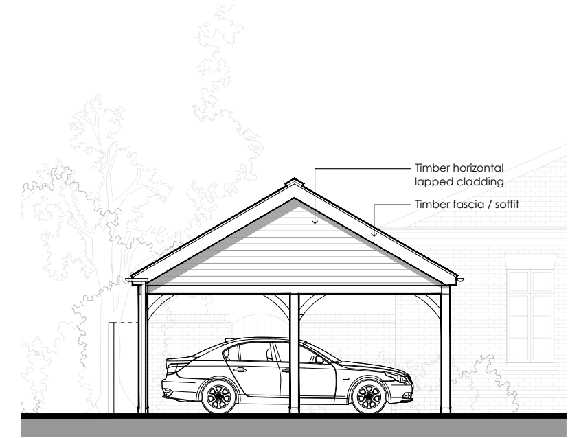
EAST ELEVATION
