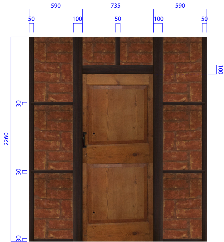
▲ Elevation (scale 1:20 @ A3)
