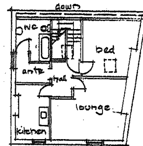
SECOND FLOOR owners flat
