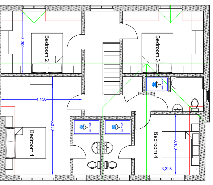
FIRST FLOOR PLOT 4
