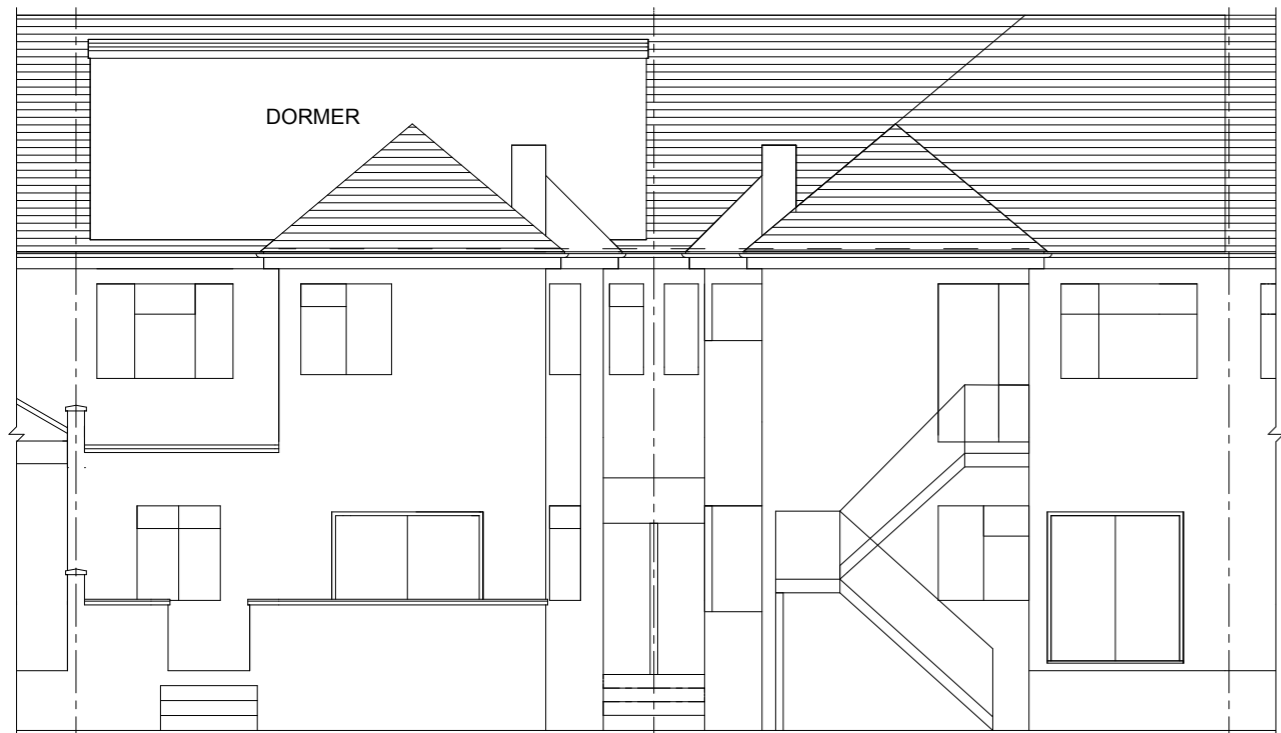
REAR ELEVATION (EXISTING)
