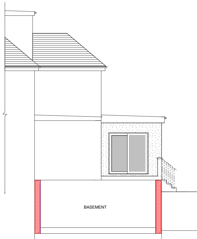
SIDE ELEVATION
