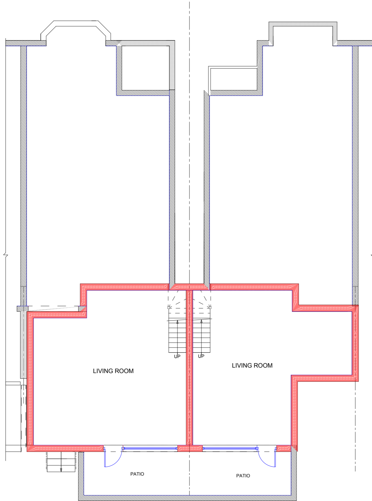
PROPOSED BASEMENT FLOOR PLAN
