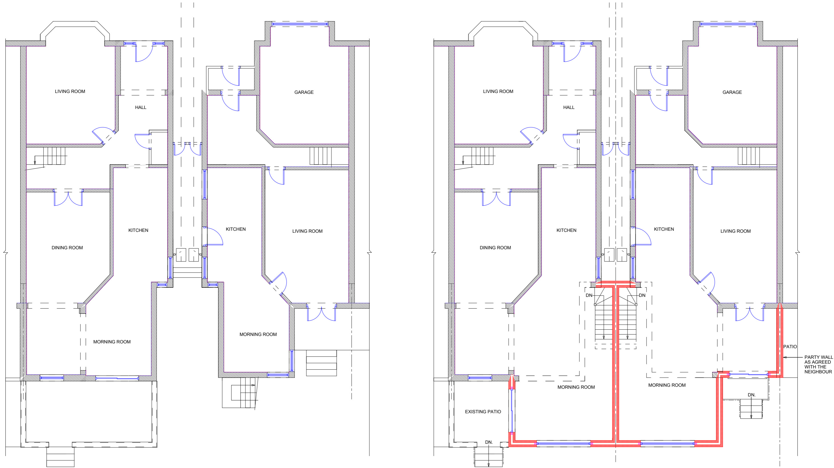
EXISTING PLAN
