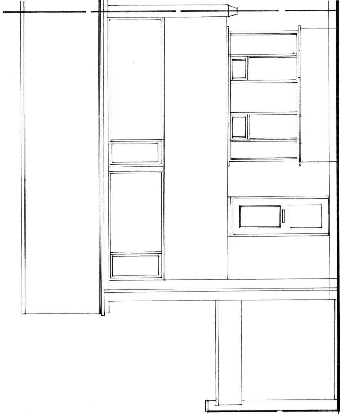
WEST ELEVATION
