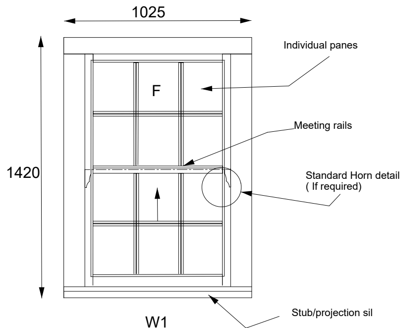
Box Casement Elevation
